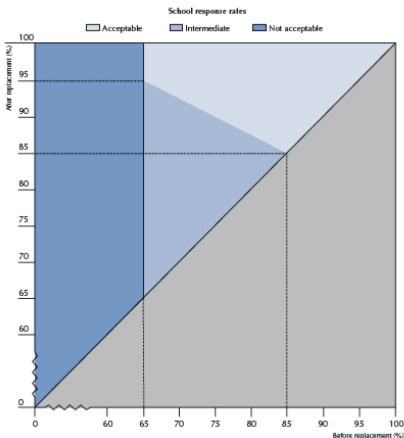
Figure 4.1: School response rate standards
