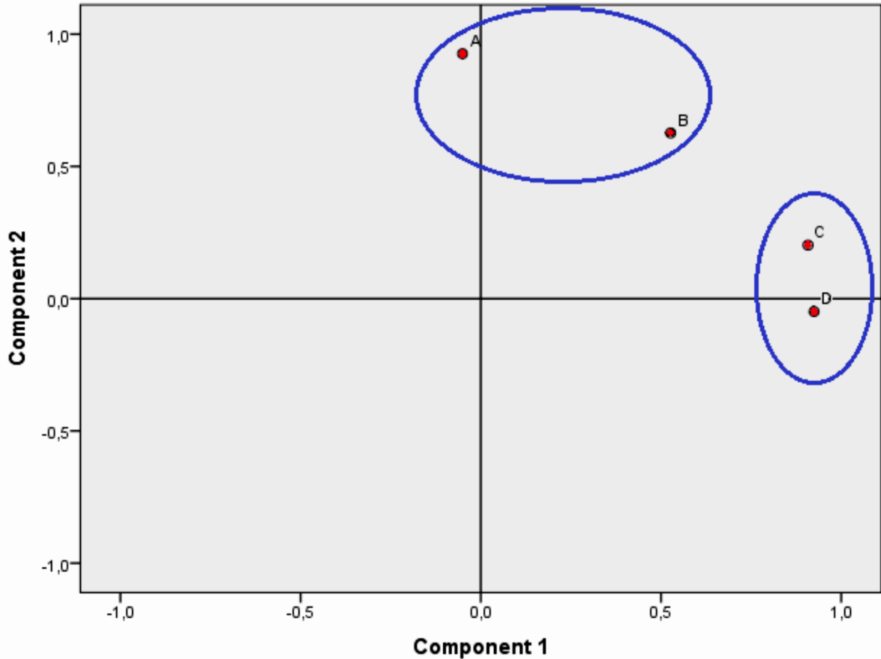
Component Plot in Rotated Space
